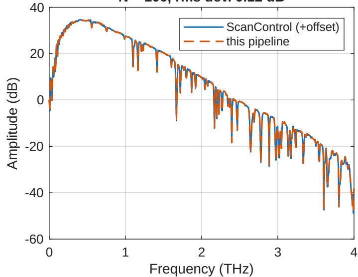
N = 100, rms dev. 0.12 dB
