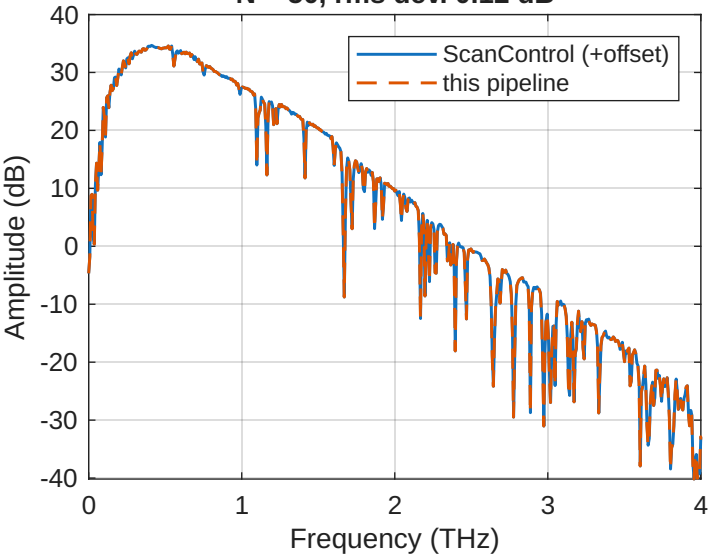
N = 50, rms dev. 0.12 dB
