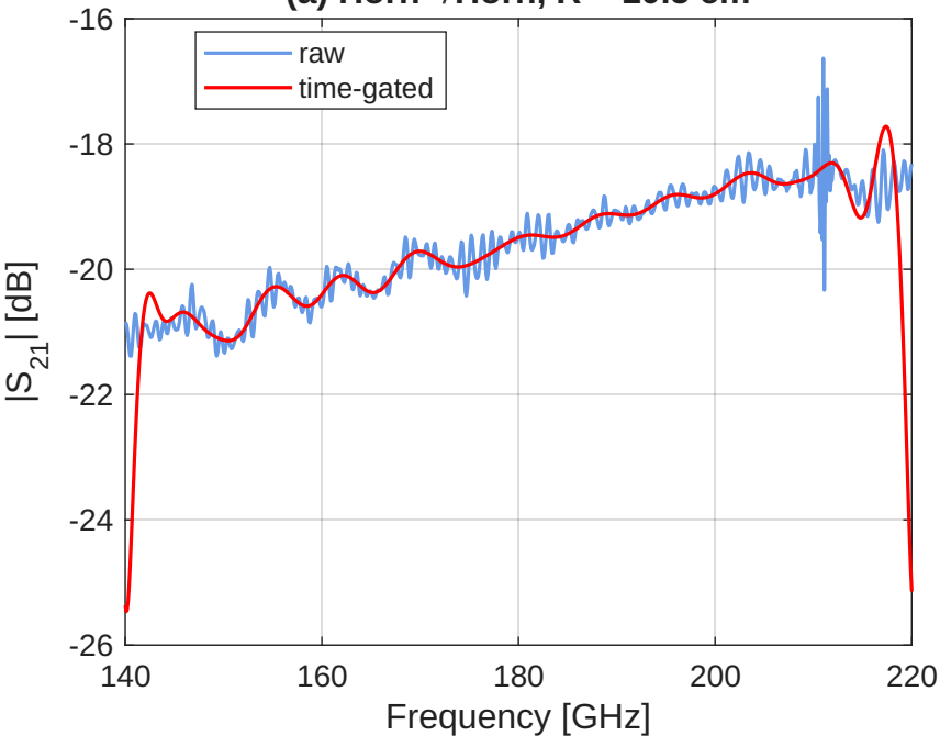
(a) Horn→Horn, R = 10.5 cm
