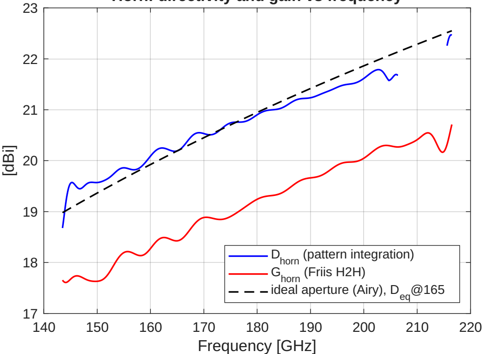
Horn: directivity and gain vs frequency
