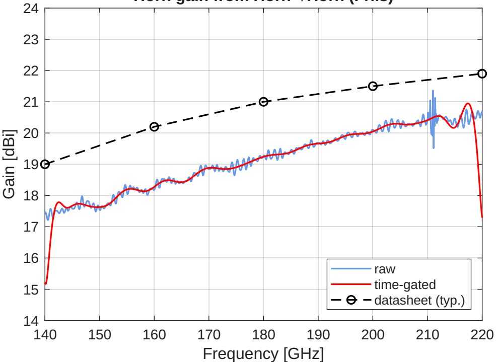
Horn gain from Horn→Horn (Friis)
