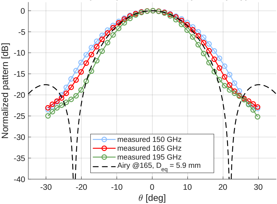
Horn H-plane pattern vs ideal aperture (Airy)
