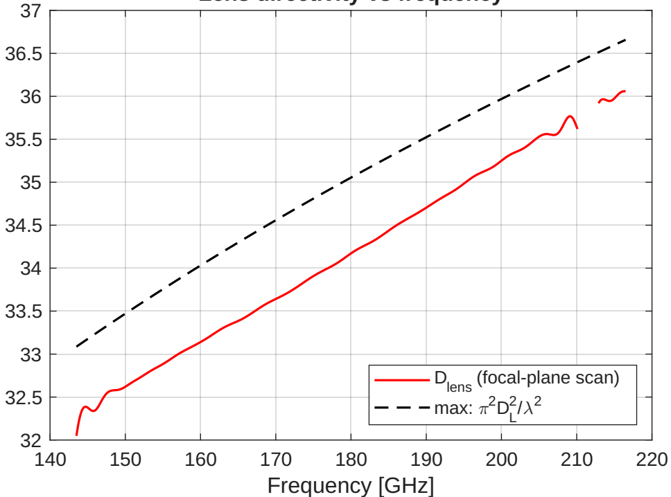
Lens directivity vs frequency
