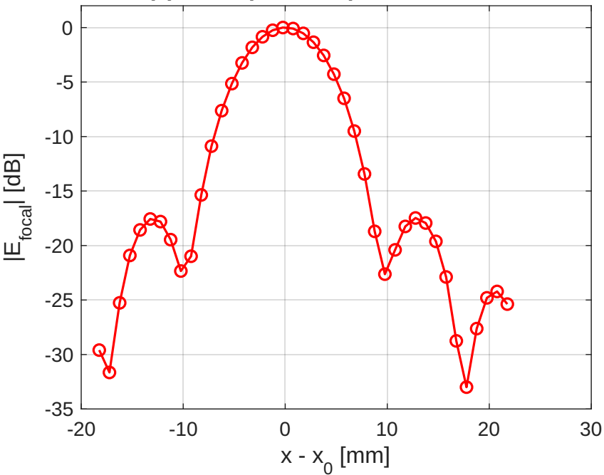
(a) Focal-plane amplitude, 165 GHz
