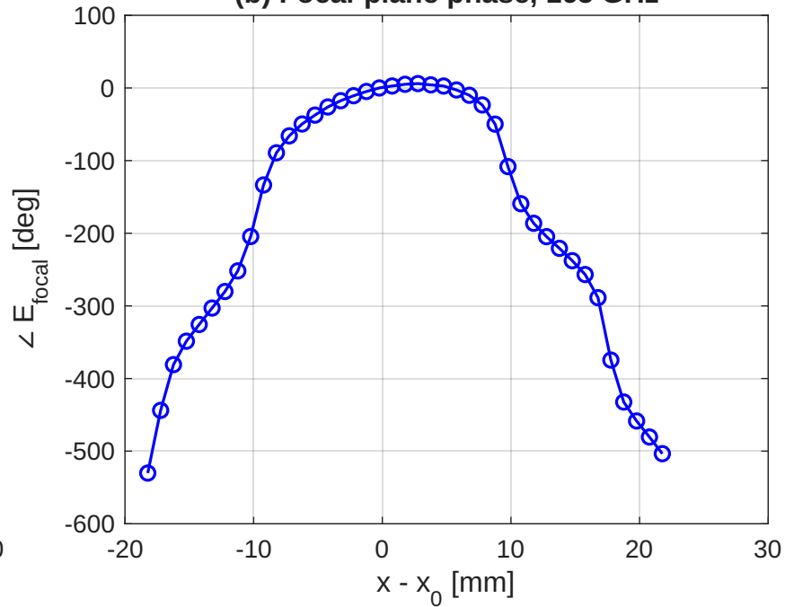
(b) Focal-plane phase, 165 GHz
