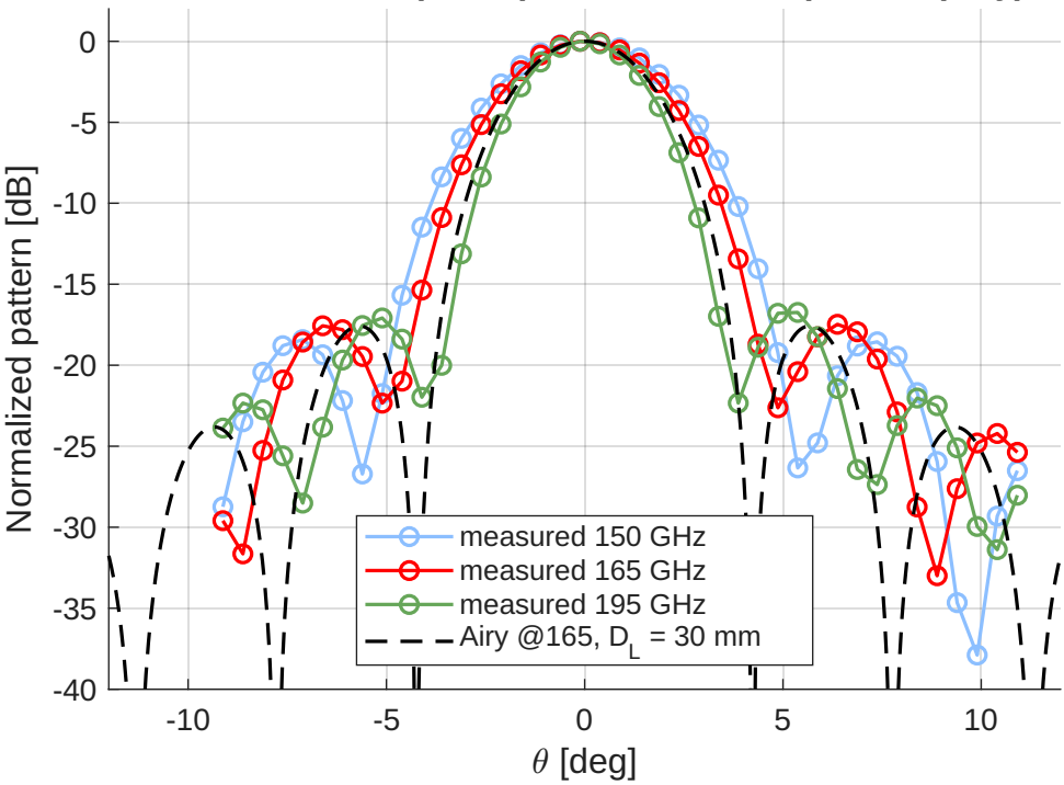
Lens antenna H-plane pattern vs ideal aperture (Airy)
