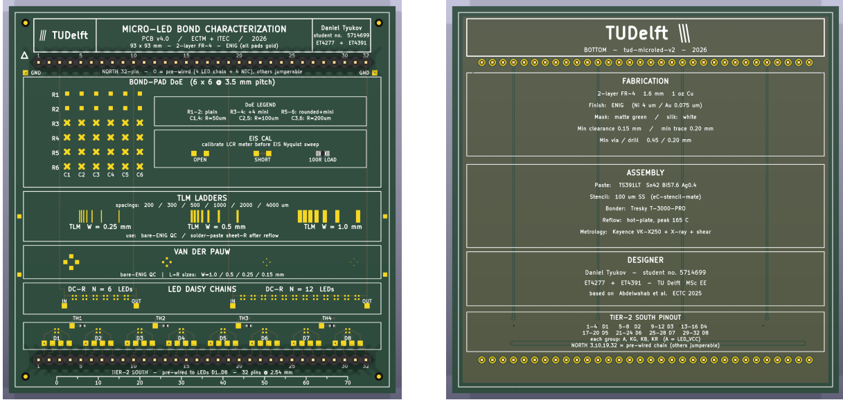
Fig. 1. v4.0.7 PCB, 93 mm \times 93 mm, two-layer FR-4, ENIG finish. Left: top side, with the DoE bond-pad array and EIS calibration block in the upper half, the TLM ladders and VDP cloverleaves in the middle, and the LED row plus NTCs at the bottom. Right: bottom side, with the fabrication / assembly / designer text blocks and the south-header pinout legend that maps the 32 cable wires to the eight LED slots.
