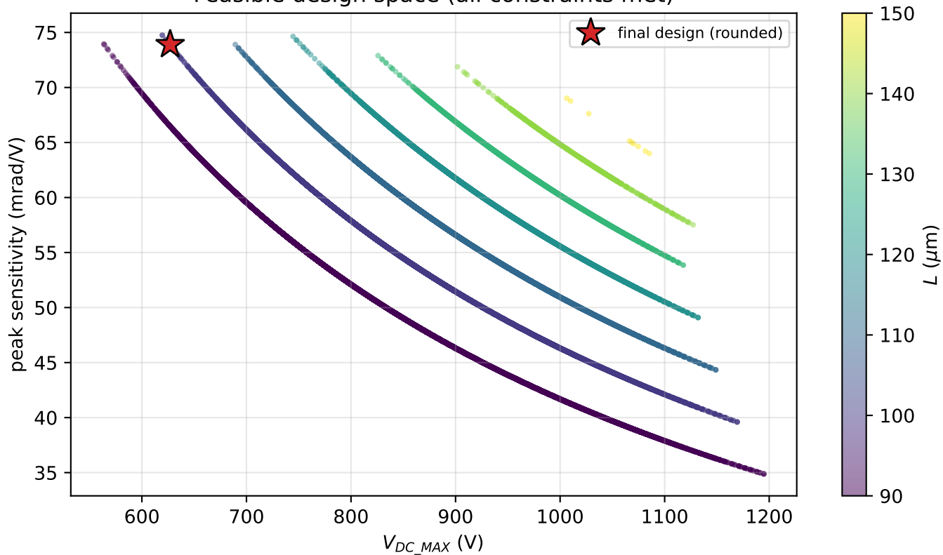
Feasible design space (all constraints met)
