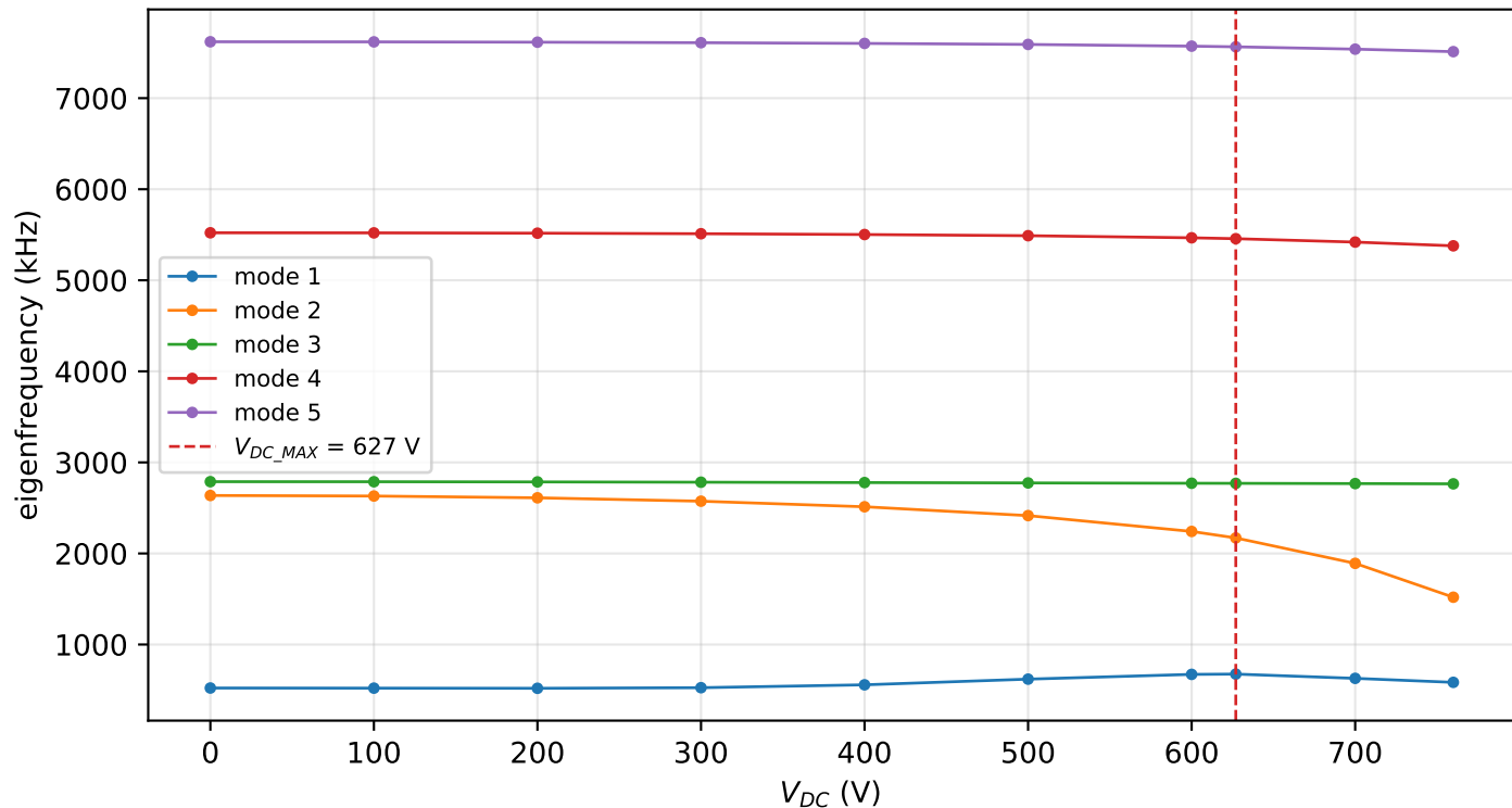
Prestressed eigenfrequencies vs bias (electrostatic softening)
