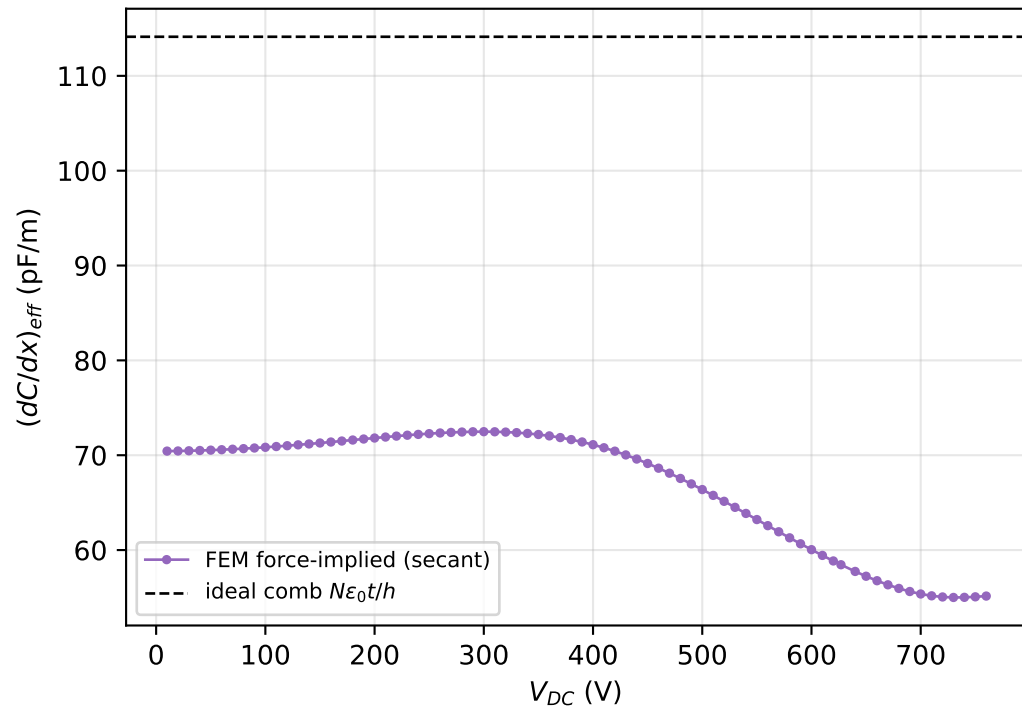
Effective comb constant: shallow-engagement deficit
