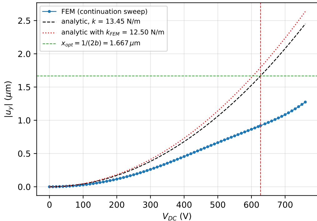
Displacement vs bias (converged through 760 V)
