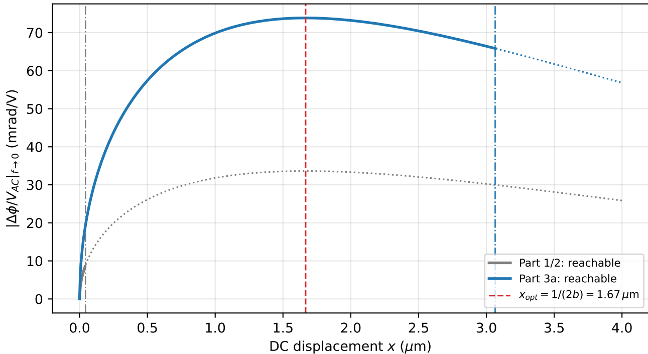
Sensitivity vs DC displacement: the travel condition
