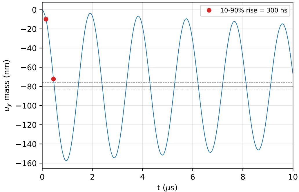
First microseconds (rise)
