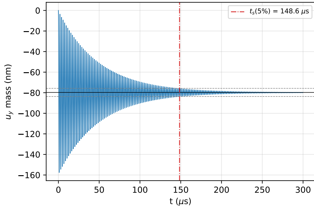
Force-step response ( 1\ \mu\text{N} ), full window
