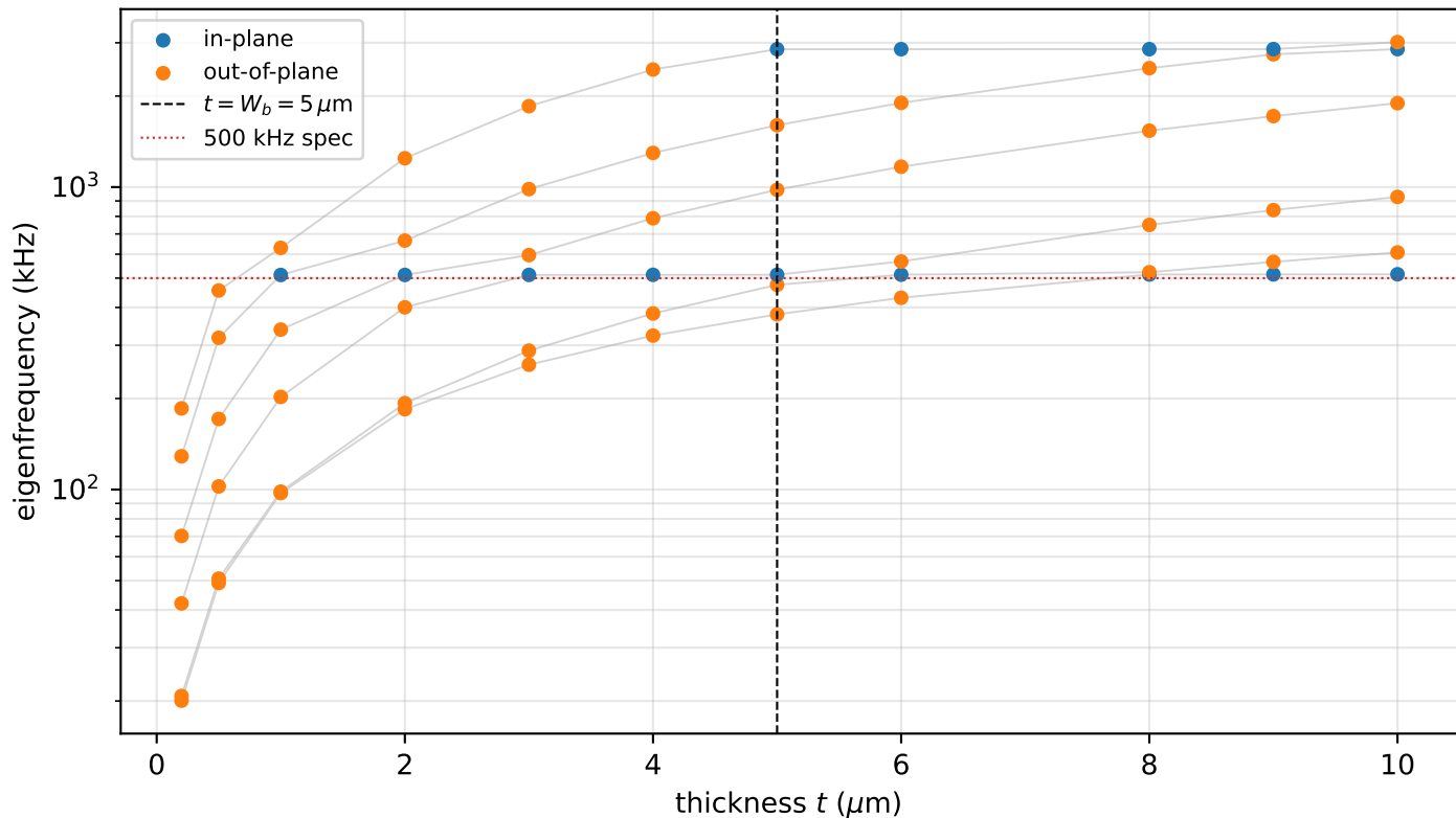
3D eigenfrequencies vs device thickness (Part-2 dims, no fingers)
