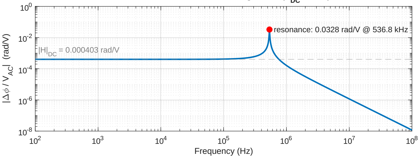
Modulation transfer function magnitude ( V_{DC} = 10\text{ V} )
