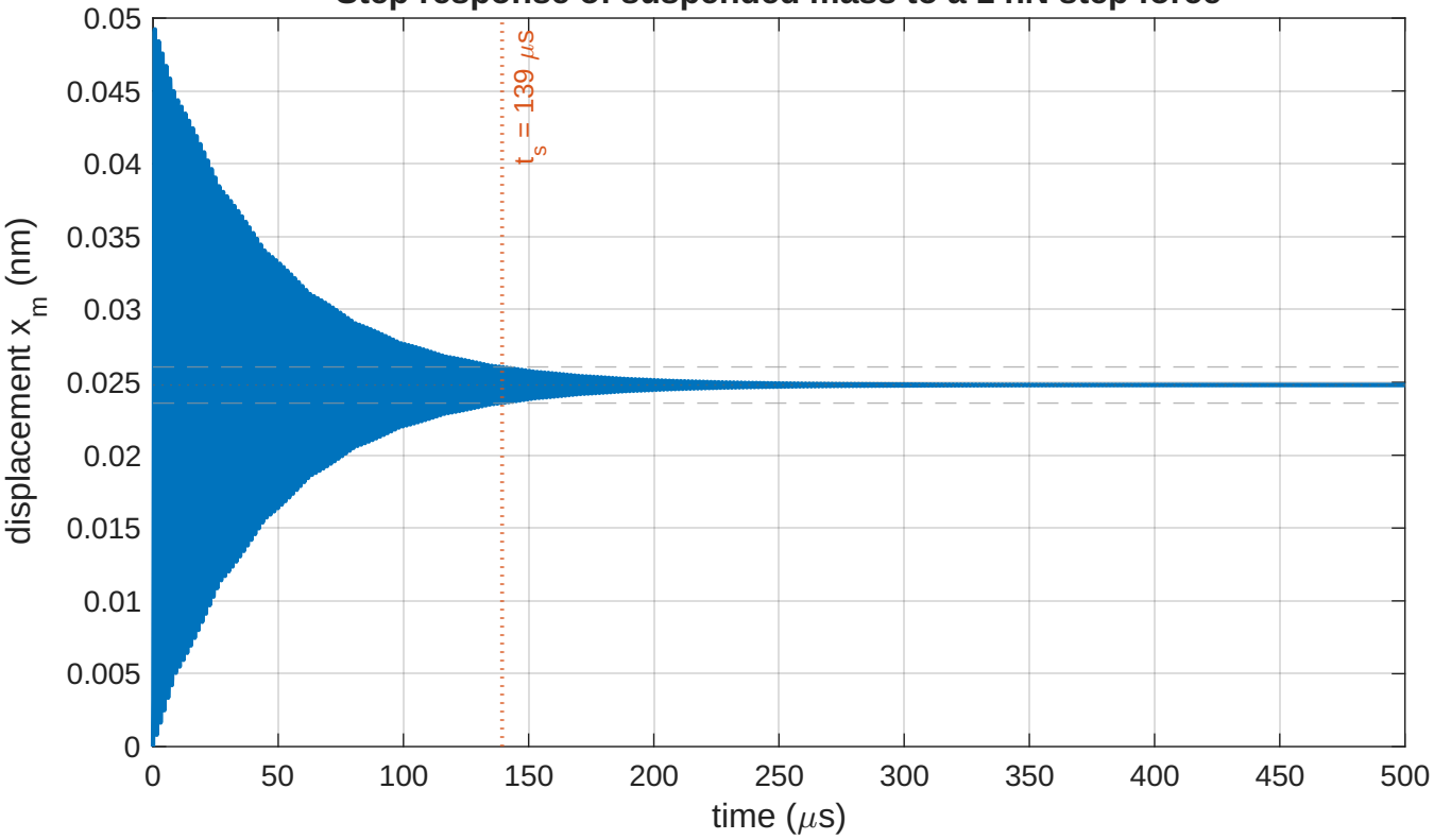
Step response of suspended mass to a 1 nN step force
