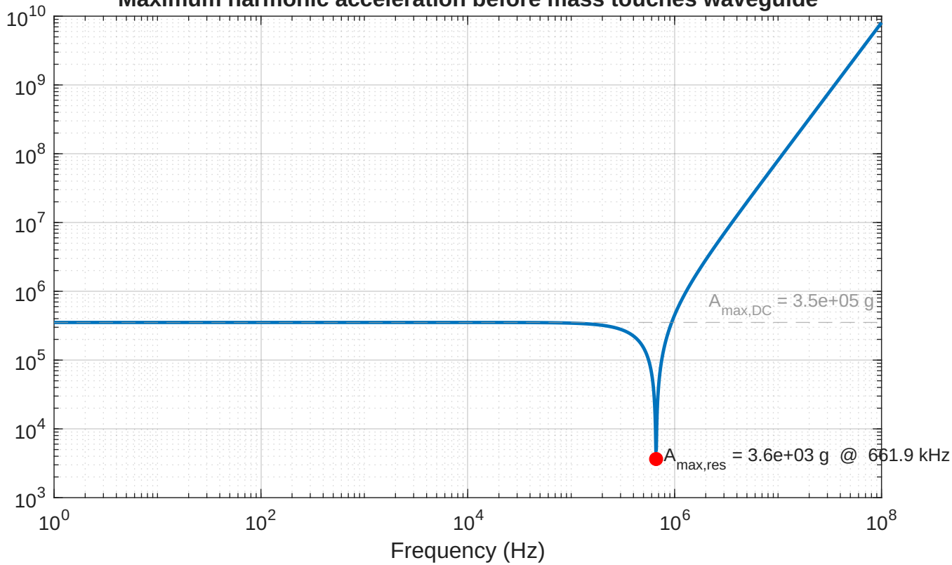
Maximum harmonic acceleration before mass touches waveguide
