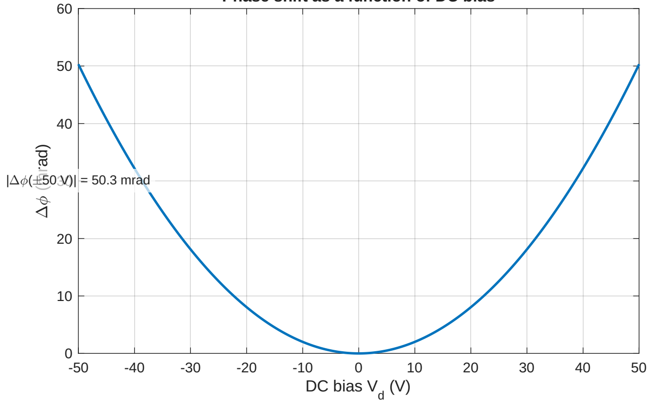
Phase shift as a function of DC bias
