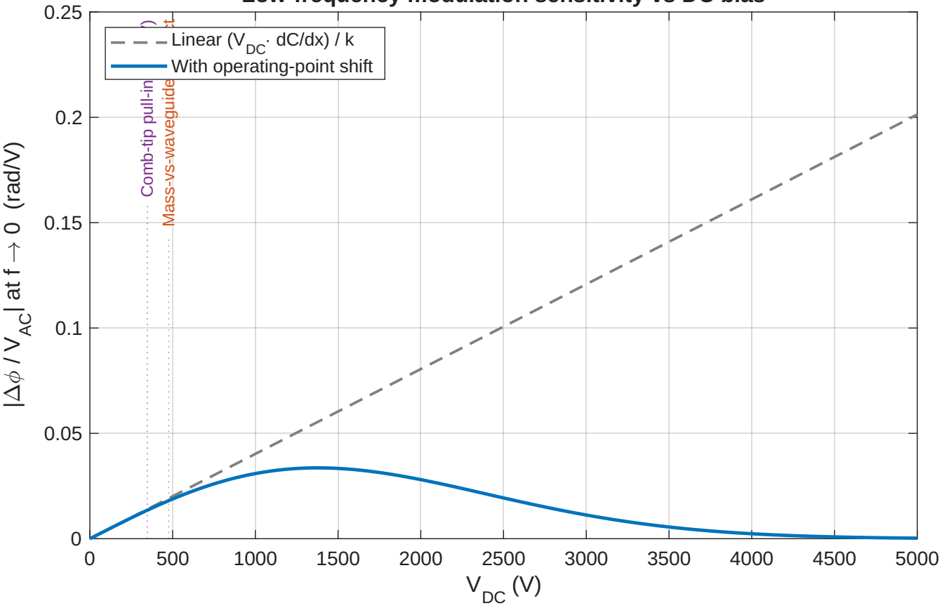
Low-frequency modulation sensitivity vs DC bias
