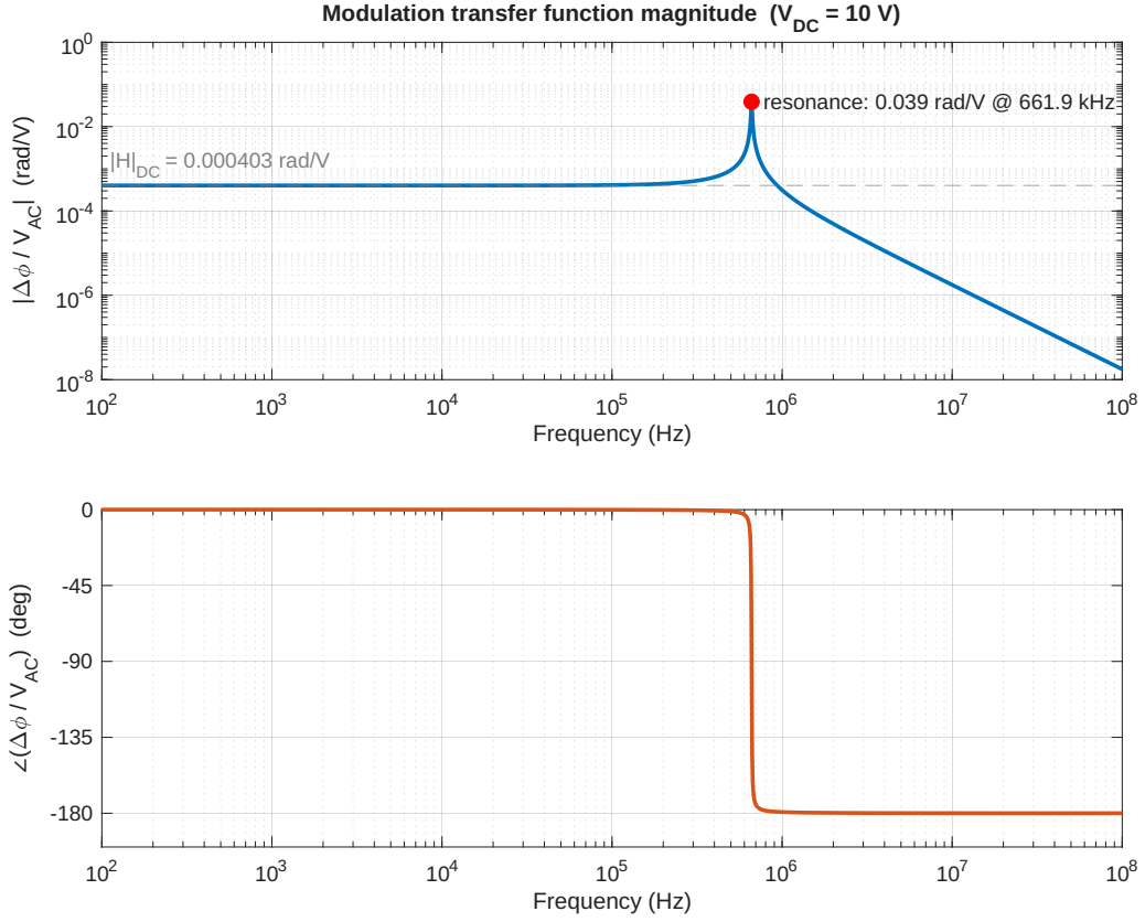
Figure 6: Bode diagram of the small-signal transfer function \Delta\phi(s)/V_{AC}(s) at V_{DC} = 10 V. The peak at f_0 \approx 662 kHz exceeds the low-frequency value by a factor of Q \approx 97 .
