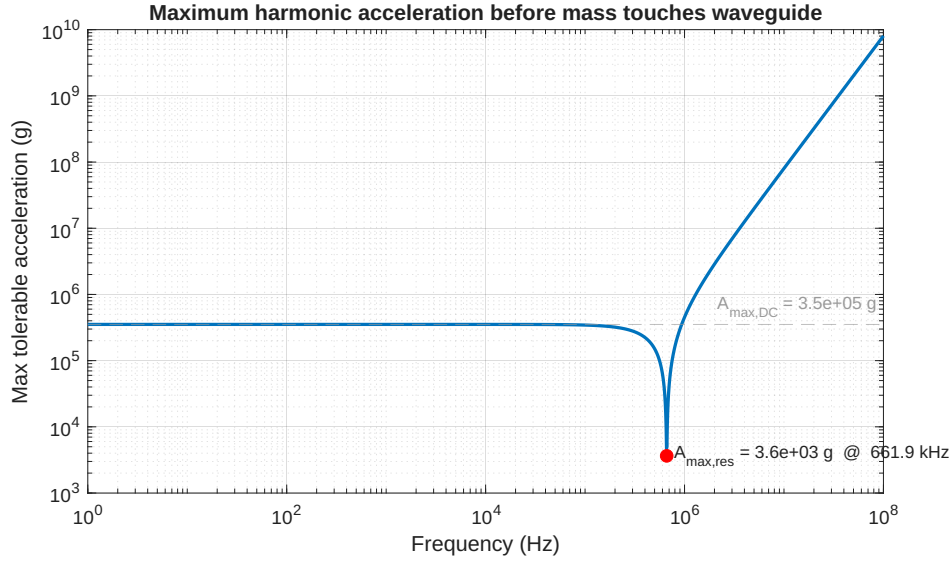
Figure 4: Maximum tolerable acceleration before the suspended mass contacts the waveguide, computed from Eq. 16. The minimum lies at f_0 \approx 662 kHz, where the device is most sensitive to mechanical excitation.
