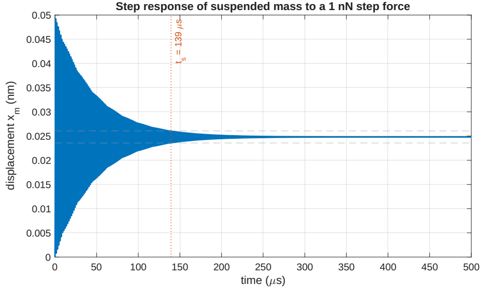
Figure 3: Step response to a 1 nN input force. The dashed lines mark the \pm 5\% band around the steady-state value F_0/k . Settling occurs after roughly t_s \approx 139 \mu\text{s} .
