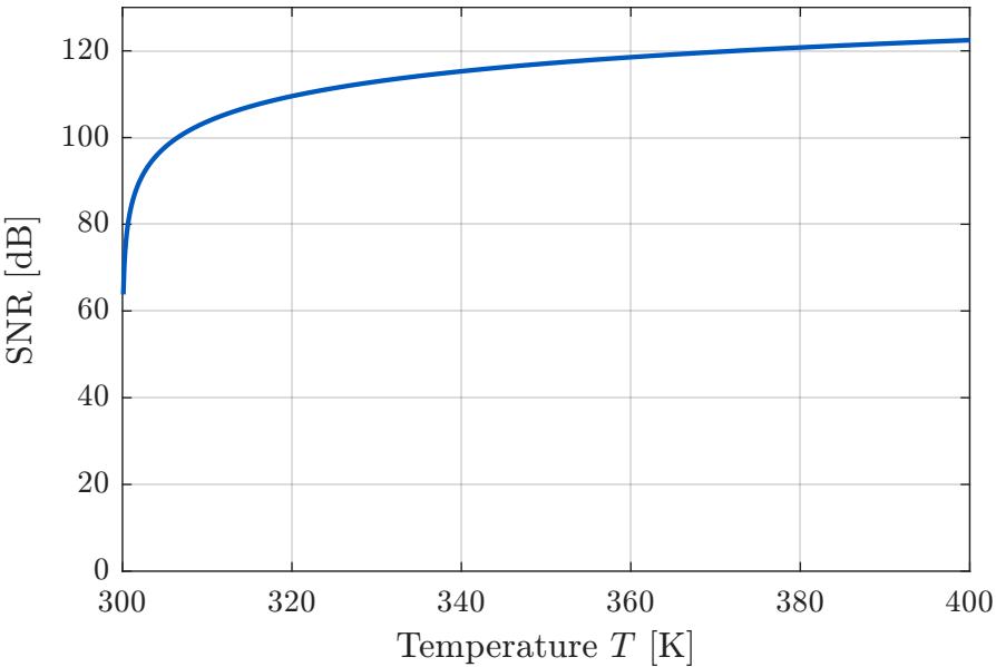
Wheatstone-bridge SNR vs. temperature (exact)
