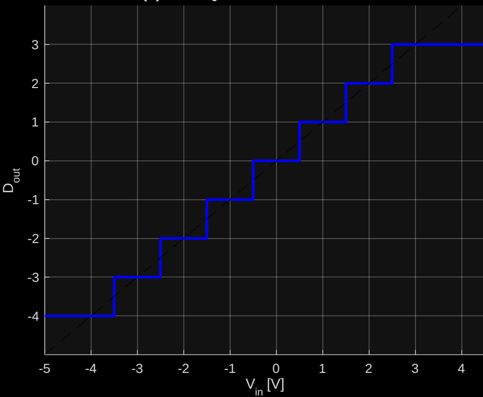
(a) Ideal Quantizer Characteristic
