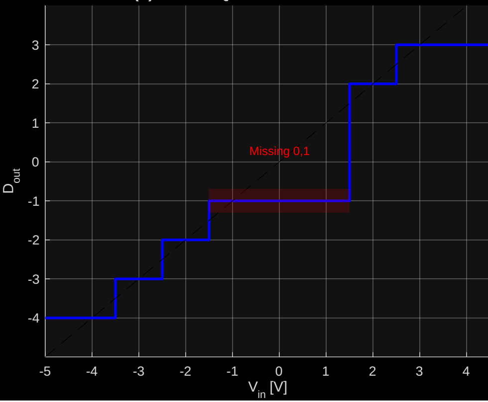
(b) Broken Quantizer Characteristic
