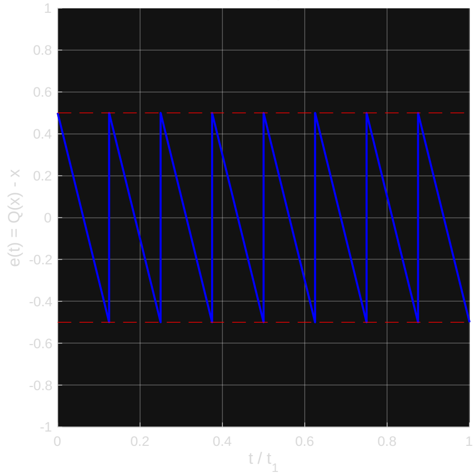
Quantization Error ( P_e = \Delta^2/12 = 0.0833 )
