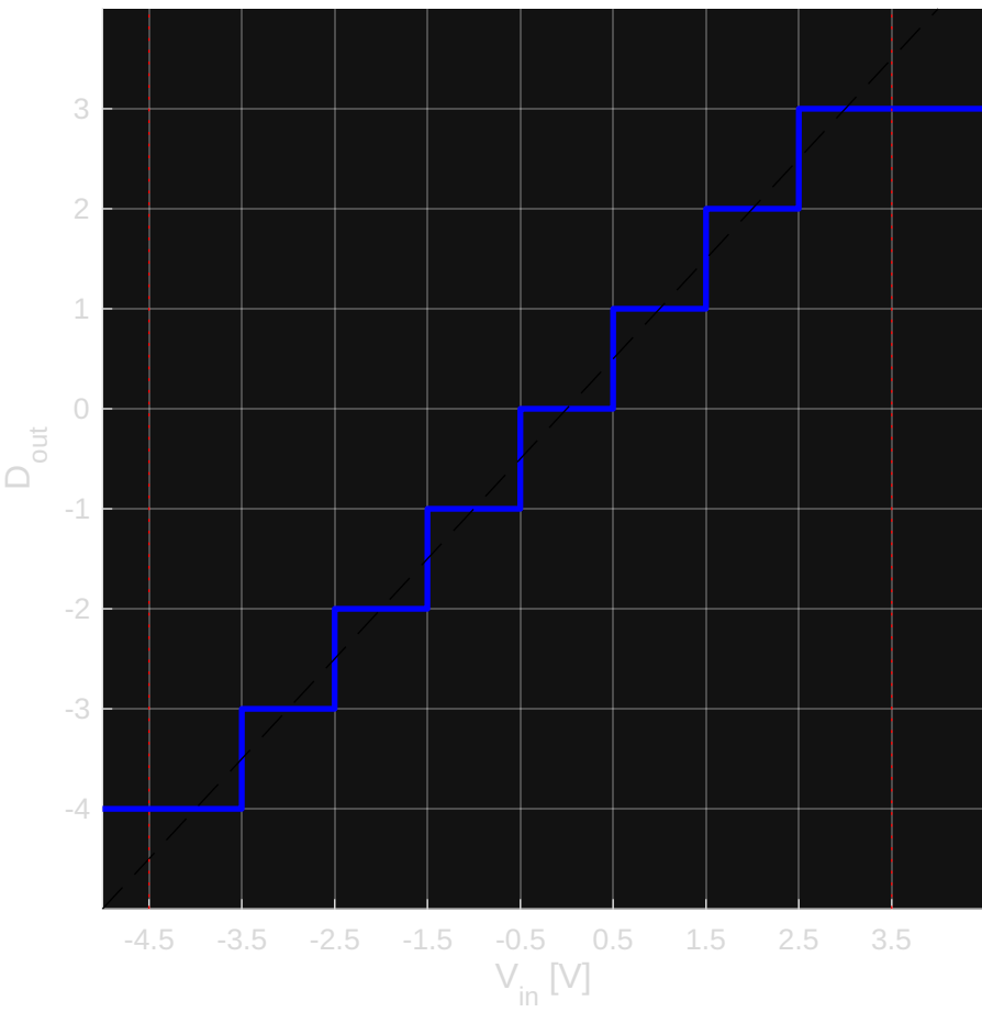
Ideal 3-bit Mid-Tread Quantizer
