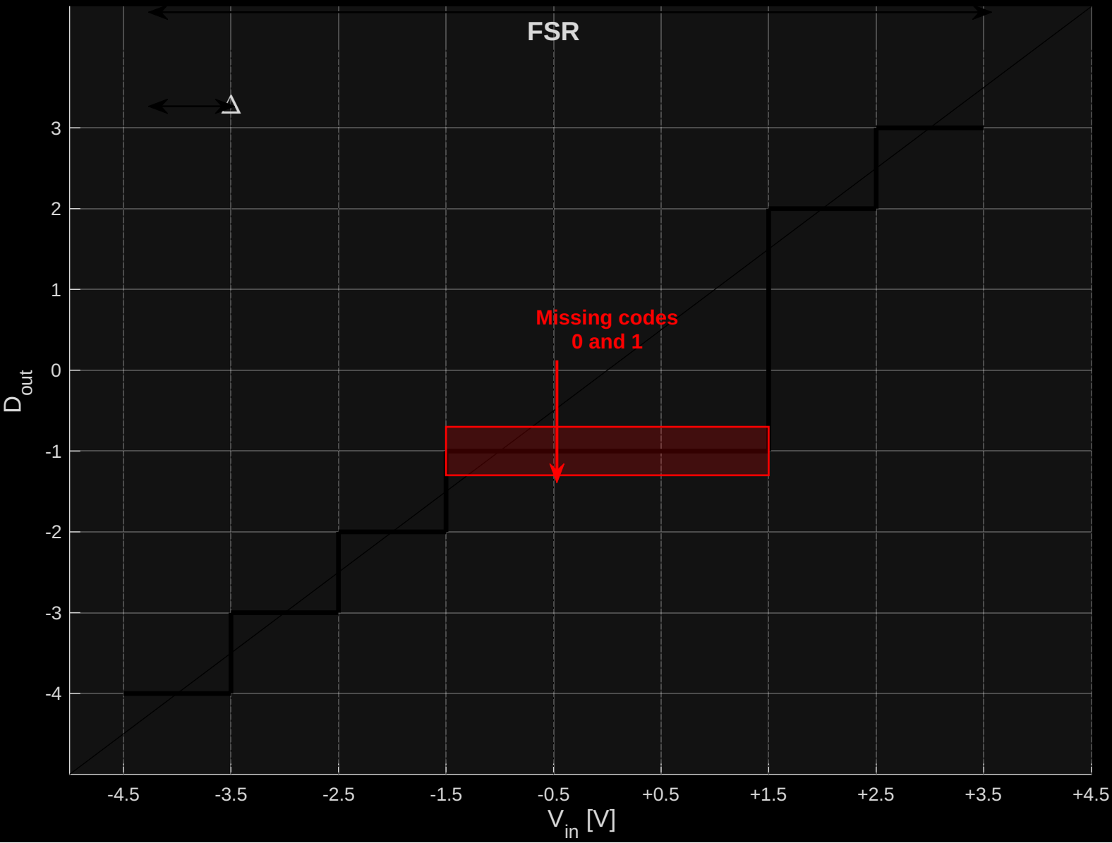
Broken 3-bit Mid-Tread Quantizer (Annotated)
