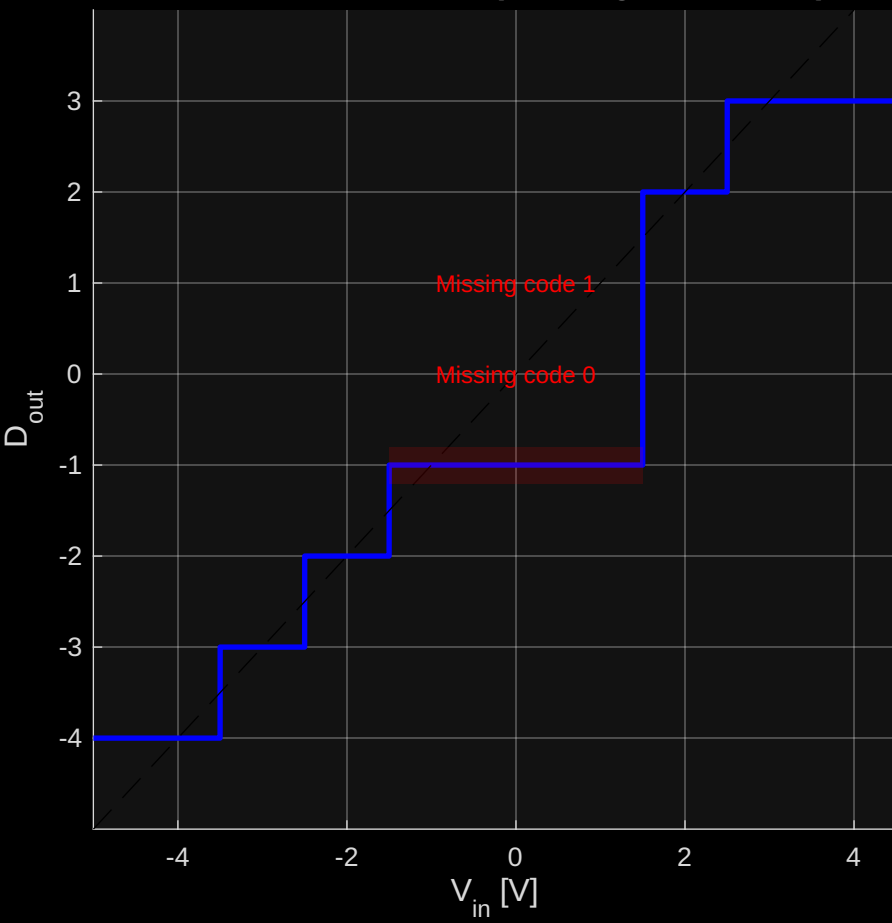
"Broken" Quantizer (Missing Codes 0, 1)
