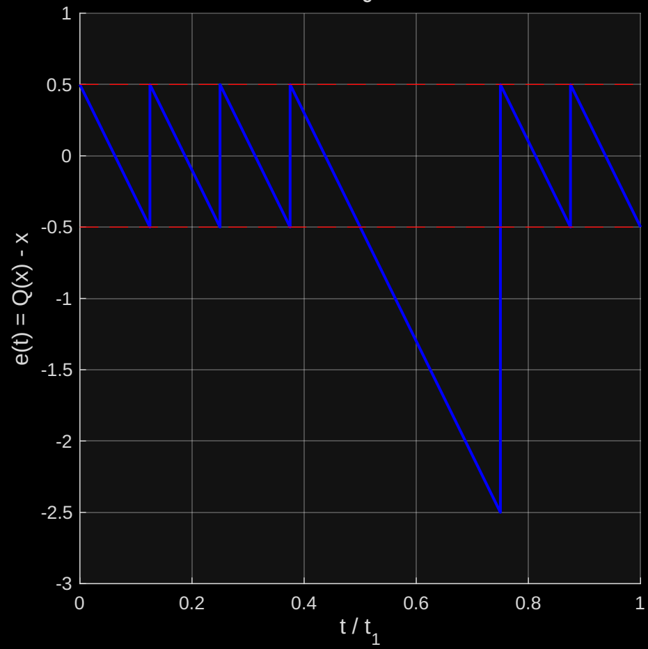
Quantization Error ( P_e = 17\Delta^2/24 = 0.7083 )
