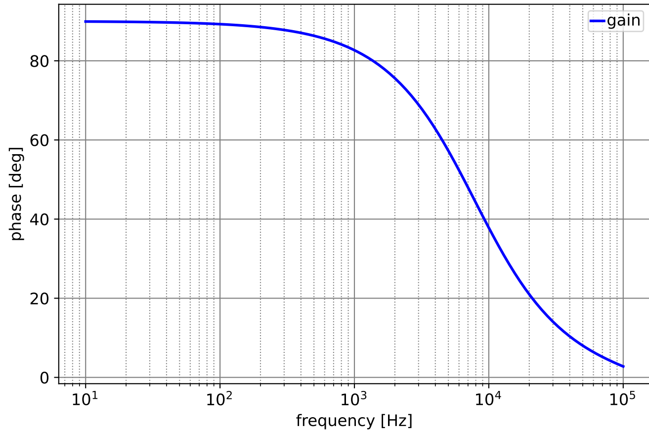
Phase characteristic
