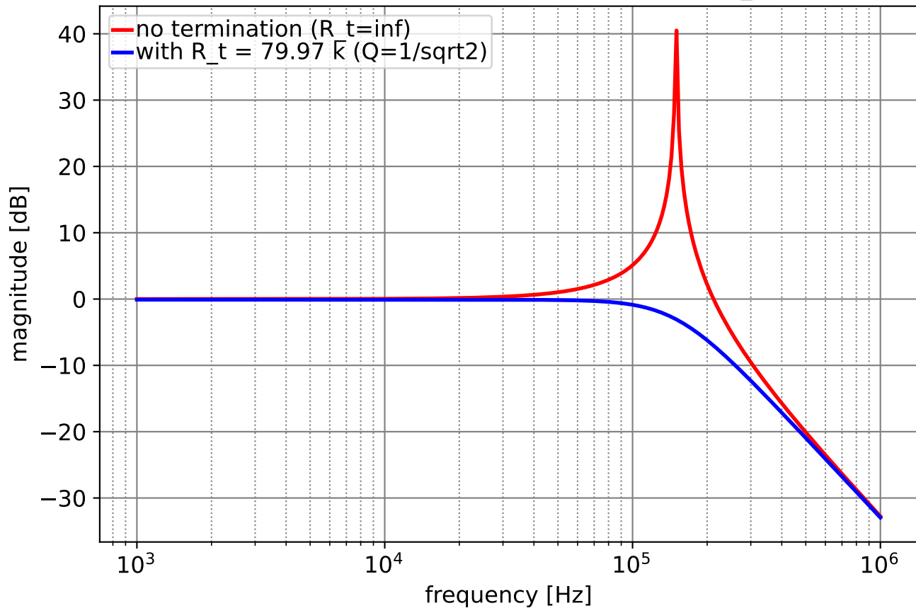
Coil self-resonance: effect of termination R_t
