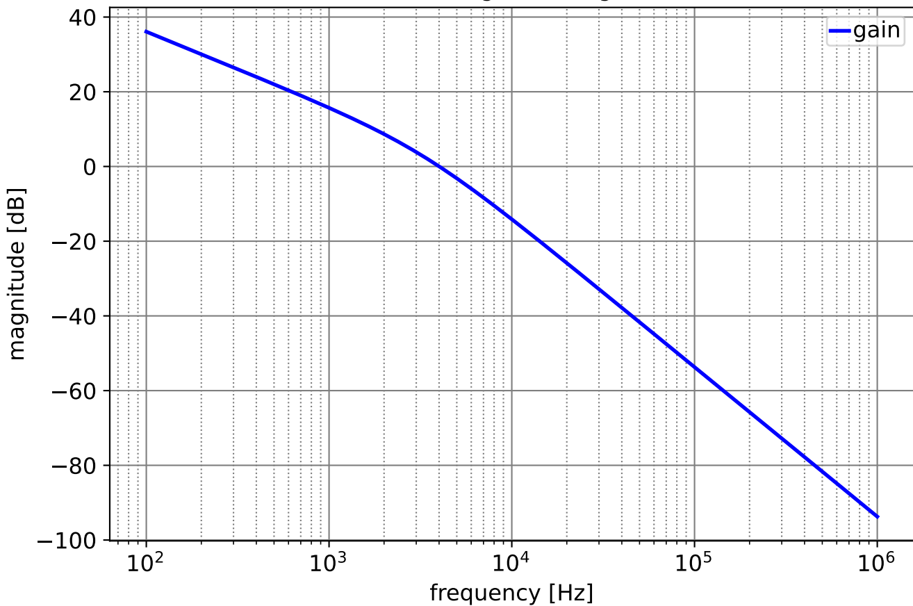
Ideal A1 integrator: magnitude
