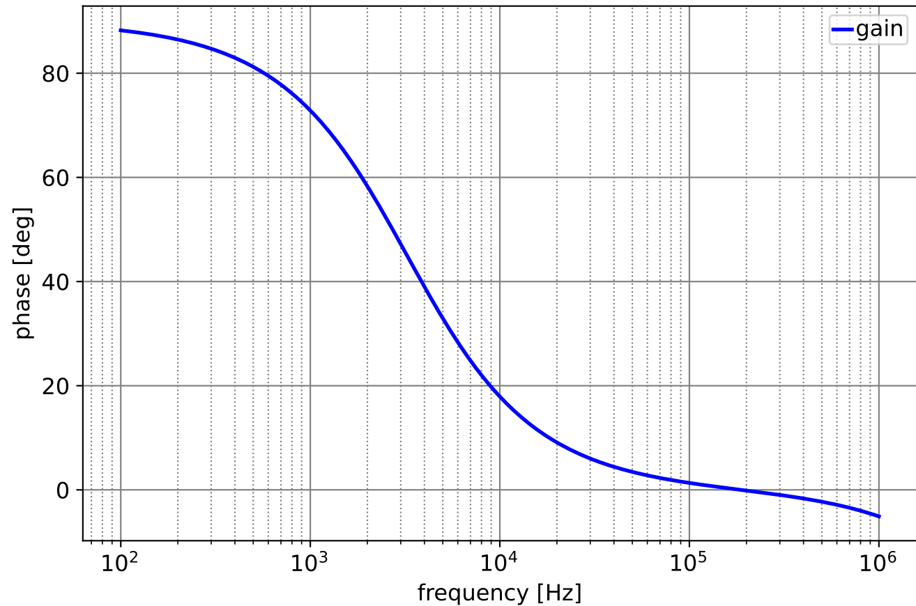
Ideal A1 integrator: phase
