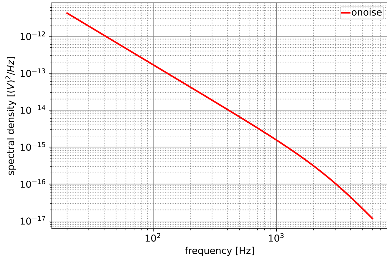
Output-referred noise spectral density
