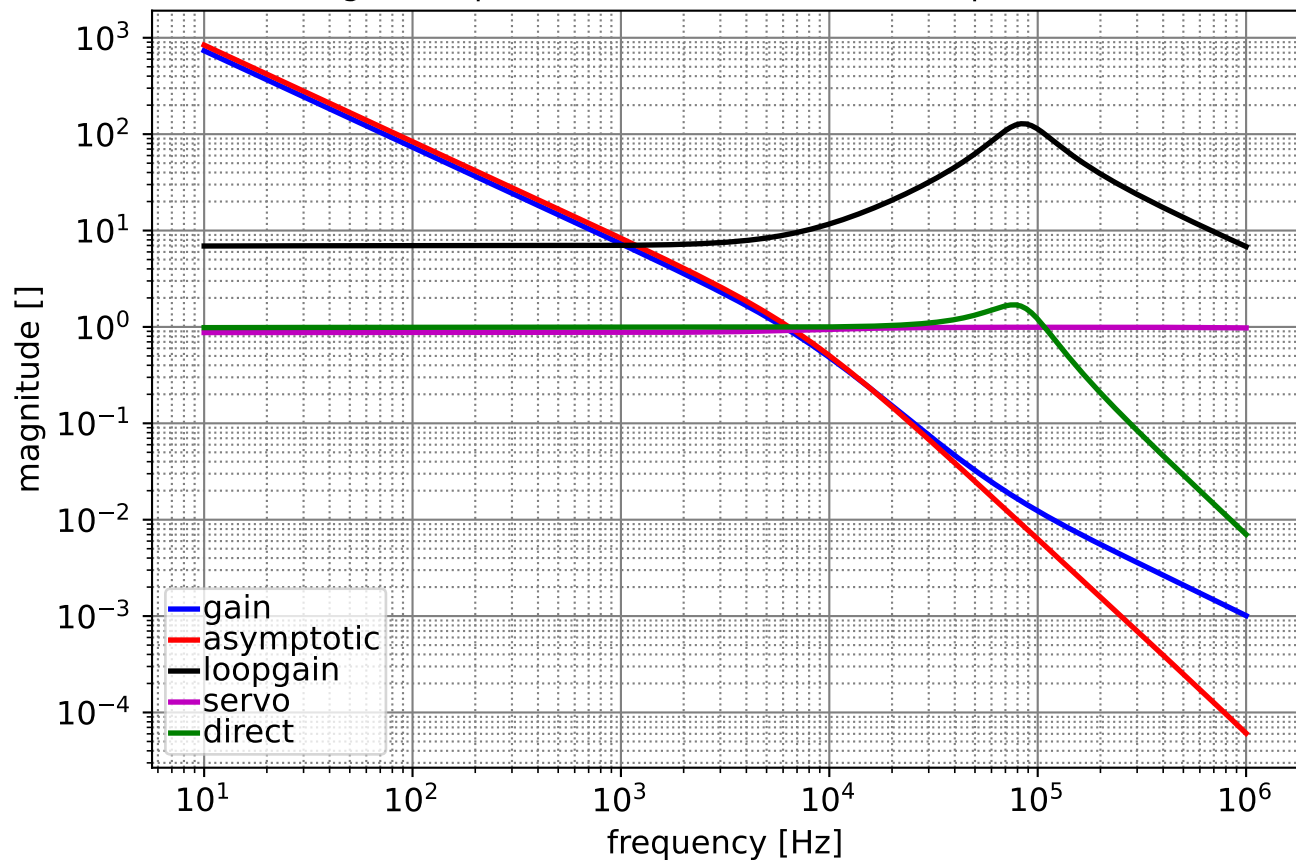
Magnitude plots cascode feedback model parameters
