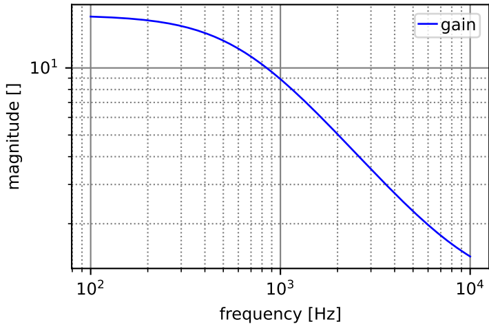
Magnitude plot gain (LF)
