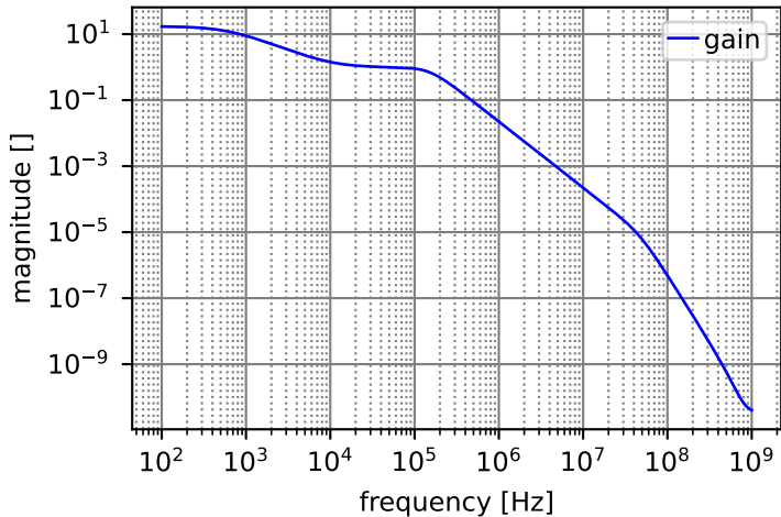
Gain of compendated dual-stage amplifier
