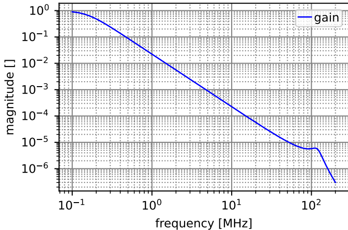
Magnitude plot gain (HF)
