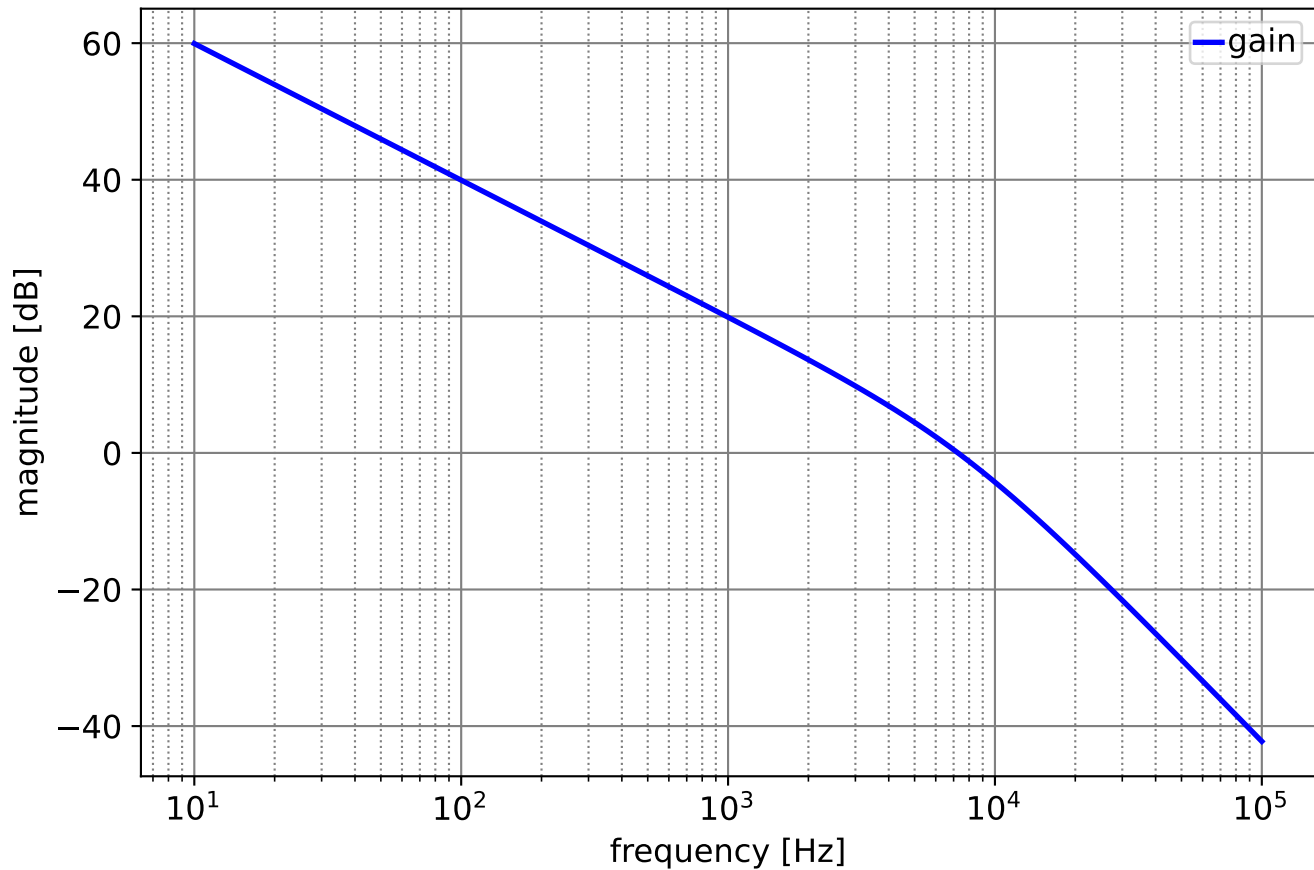
dB magnitude characteristic
