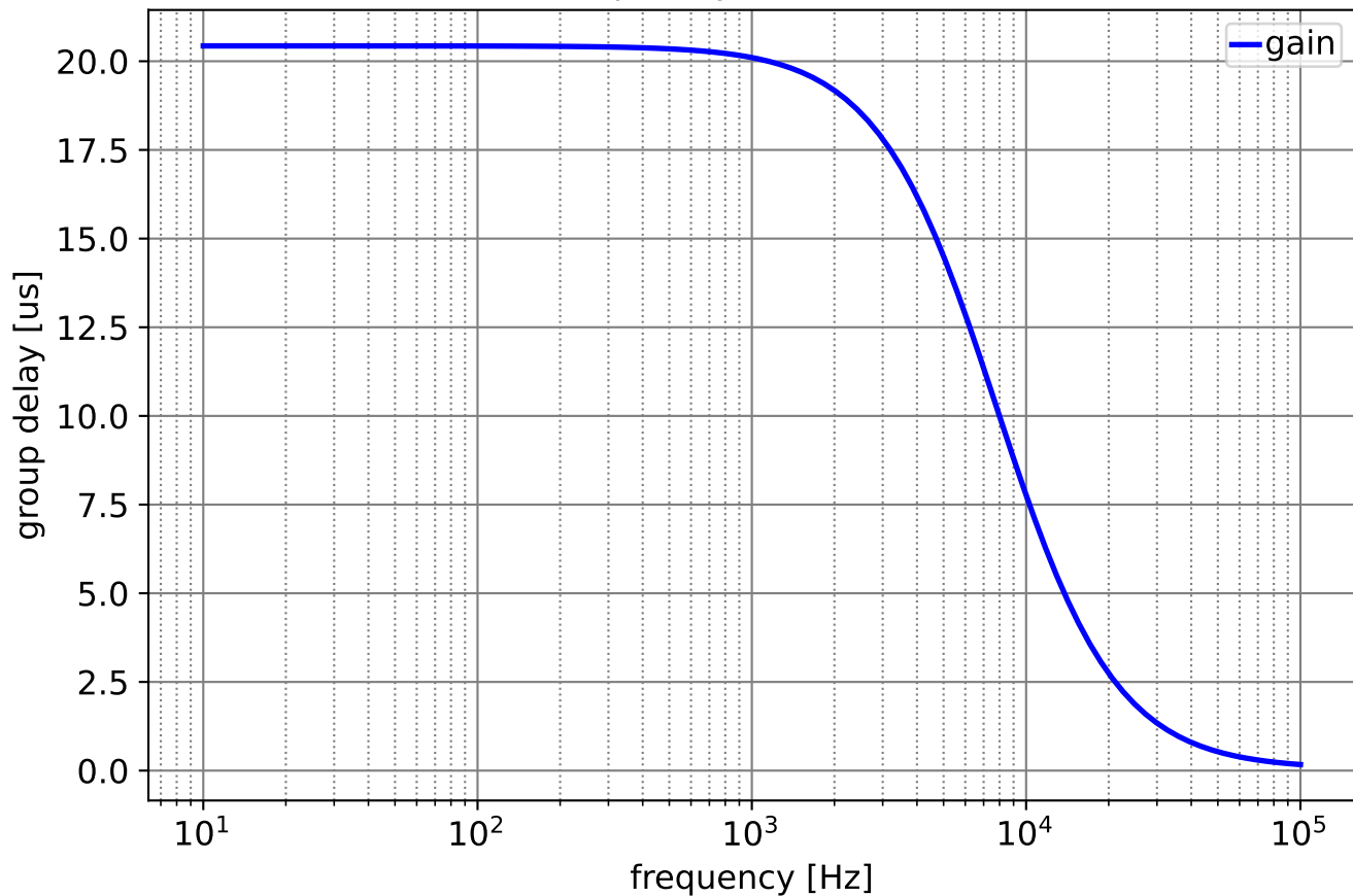
Group delay characteristic
