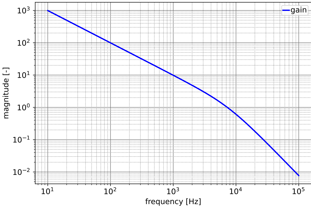
Magnitude characteristic
