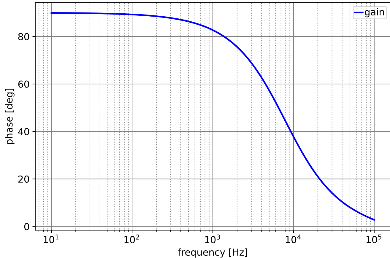
Phase characteristic
