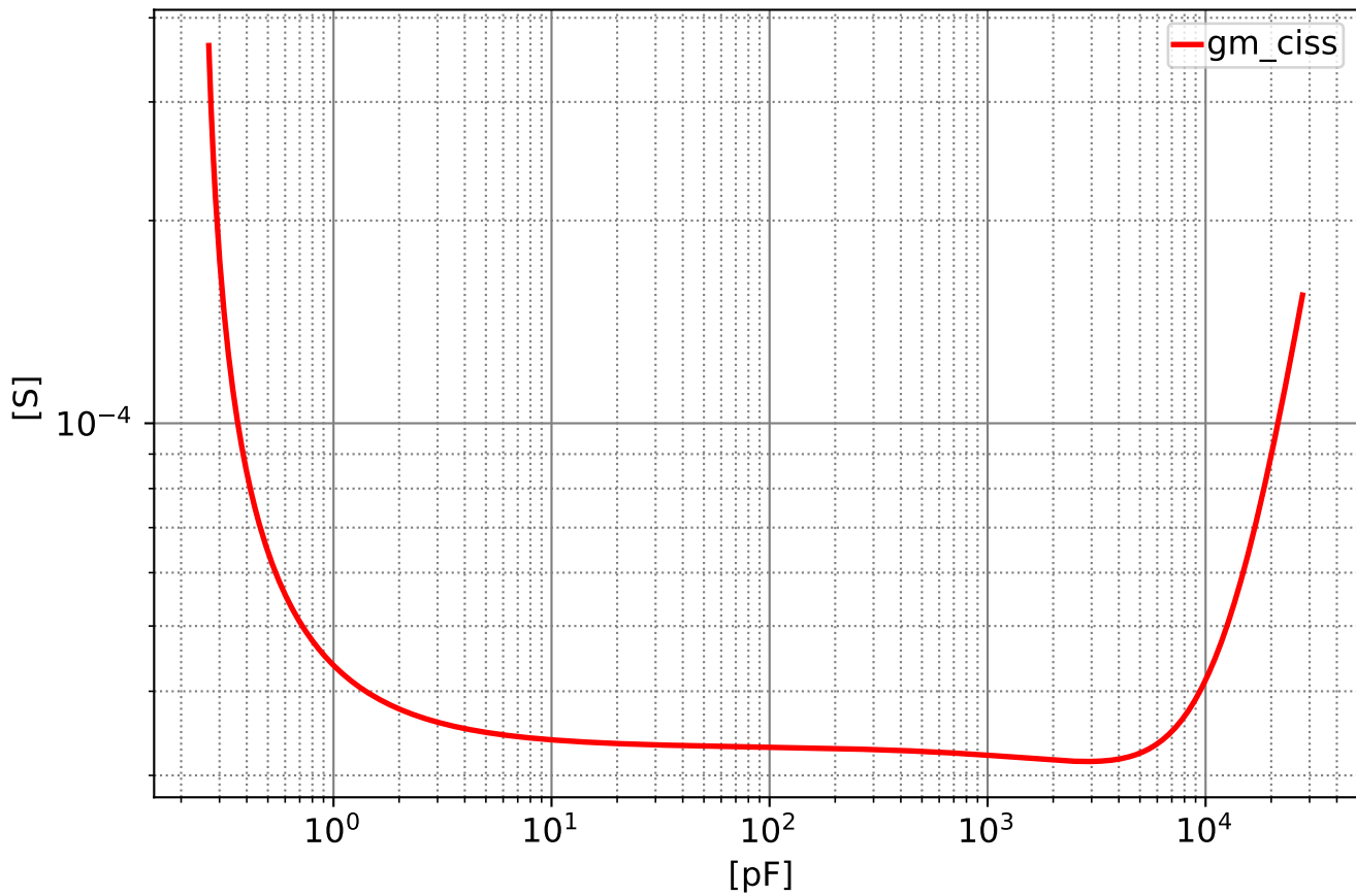
Required g_m versus c_{iss}
