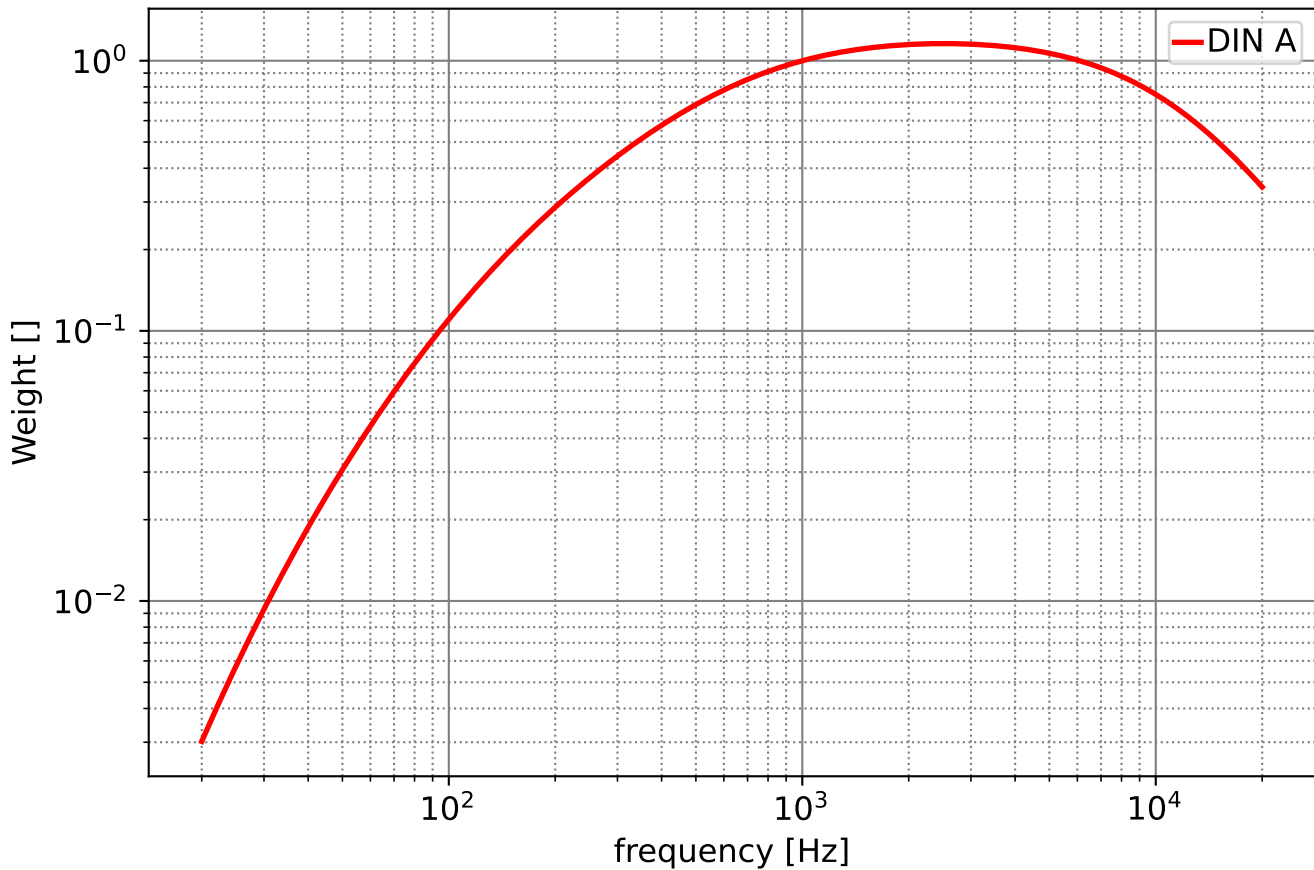
DIN A normalized at 1kHz
