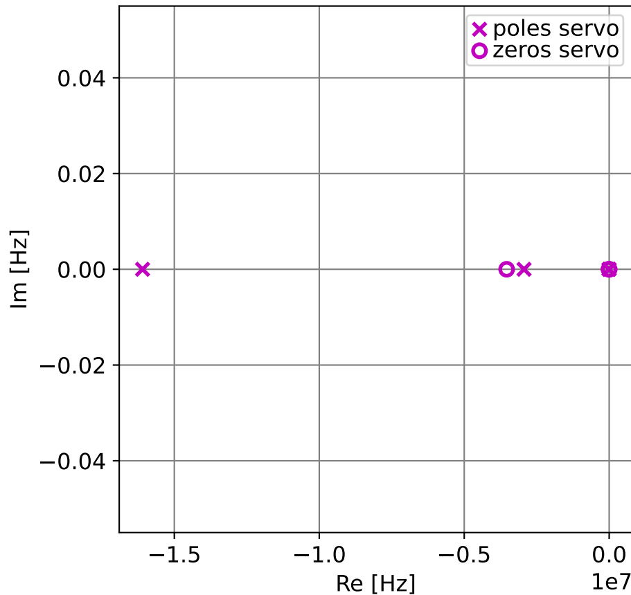
PZplotservo
