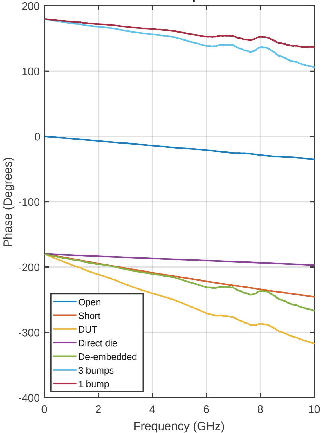
Phase Response
