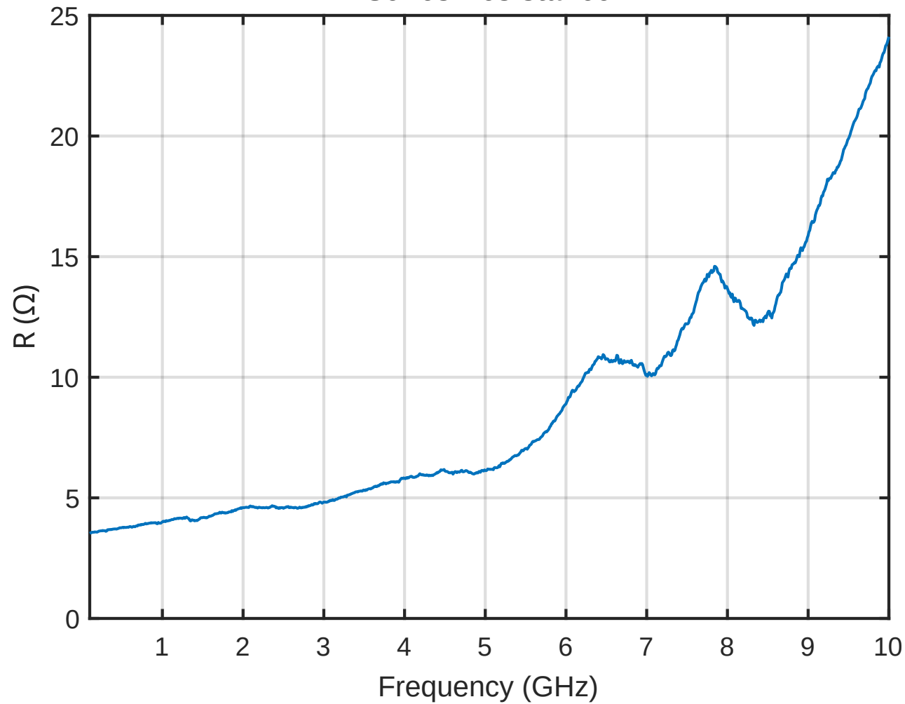
Series Resistance
