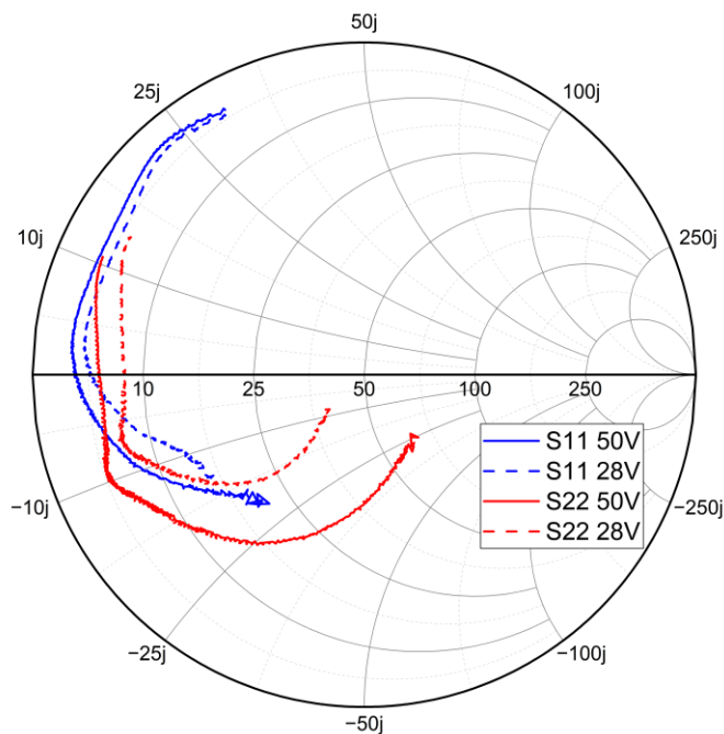
S11 &amp; S22 0.4-8 GHz
