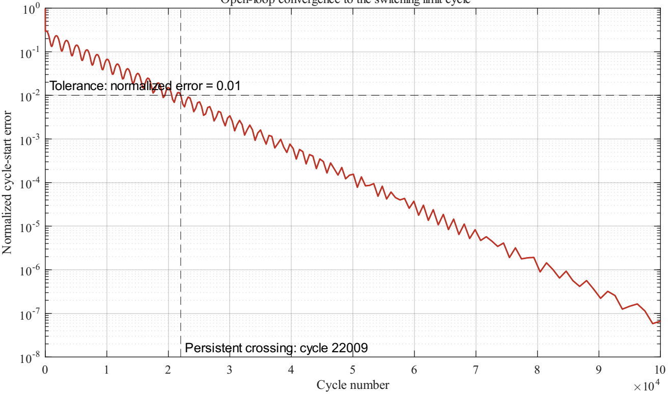
Open-loop convergence to the switching limit cycle
