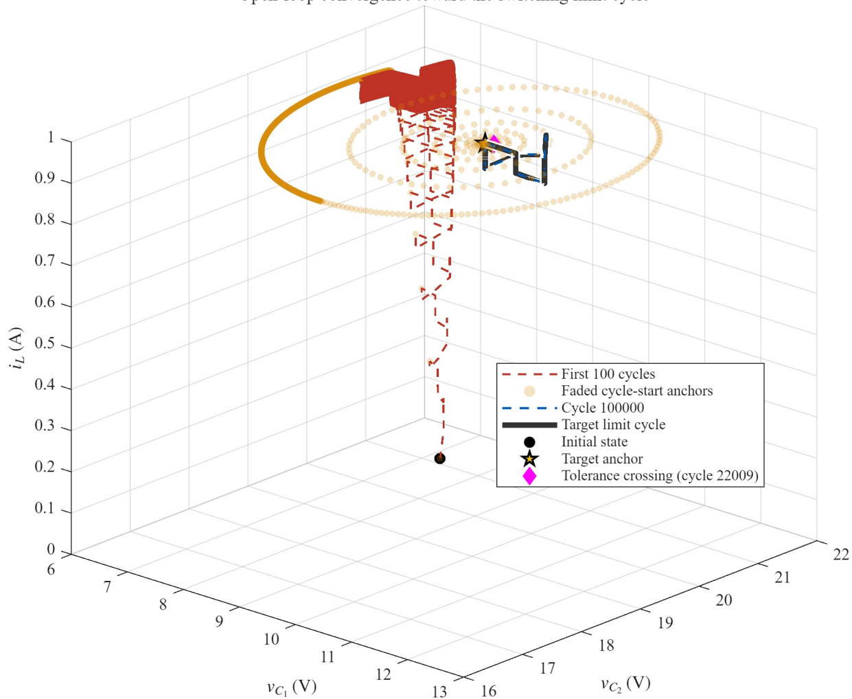
Open-loop convergence toward the switching limit cycle
