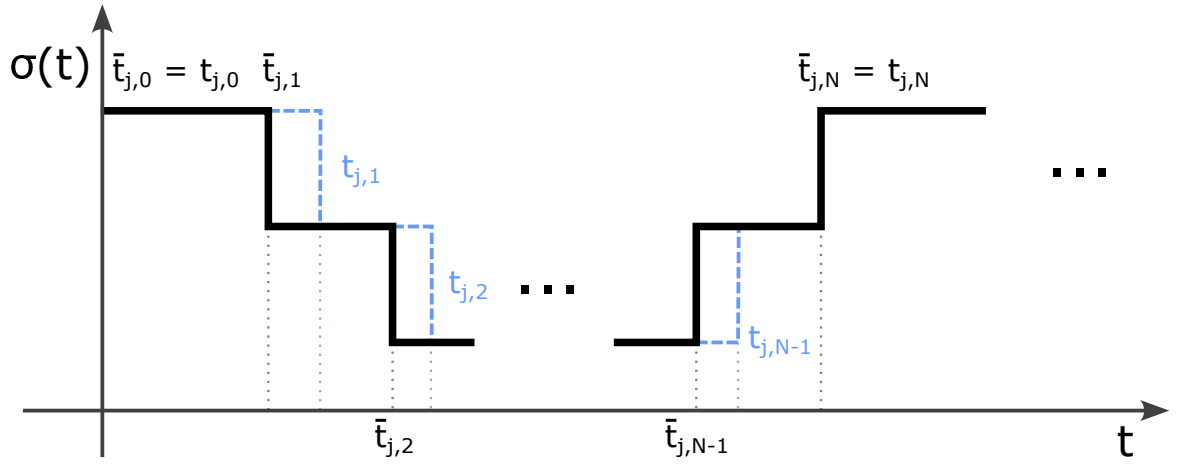
FIGURE 4.1 – Input signals
