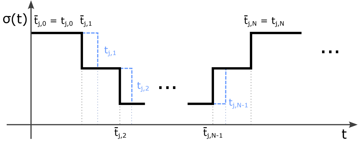
FIGURE 4.1 – Input signals
