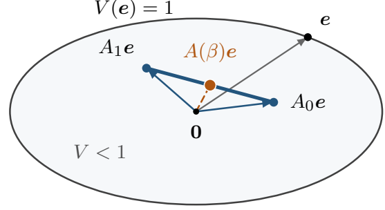
Figure 2 Common- P schematic in error coordinates. Both endpoint images lie inside the unit level set of V . Every intermediate image A(\beta)e lies on the segment joining them.
